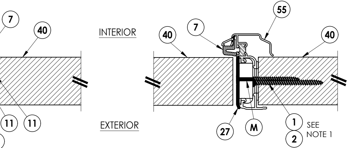
2 3 HORIZONTAL CROSS SECTION Outswing shown - inswing also approved
