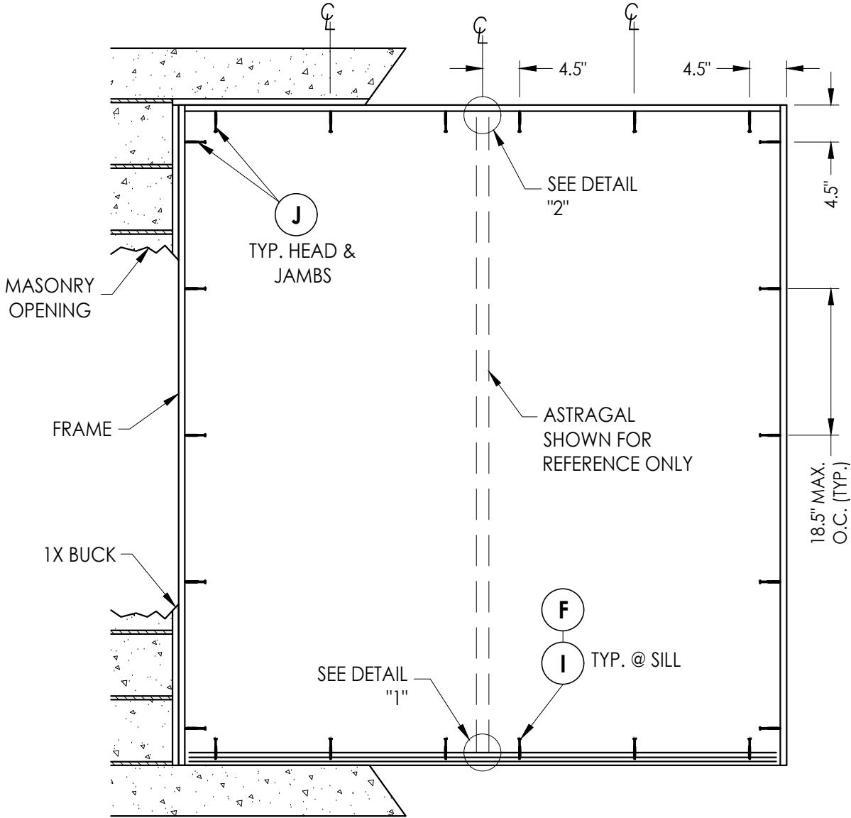
FRAME ANCHORING Masonry 1X buck construction
